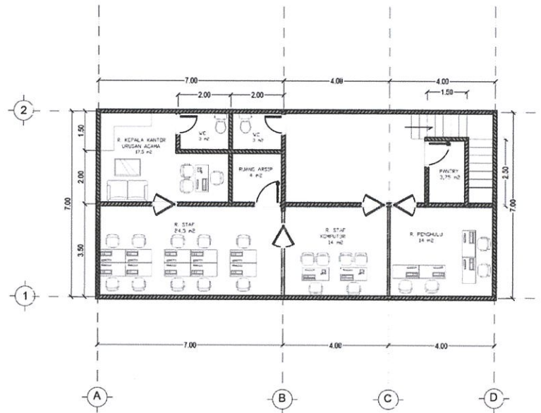
Denah Lantai 2
